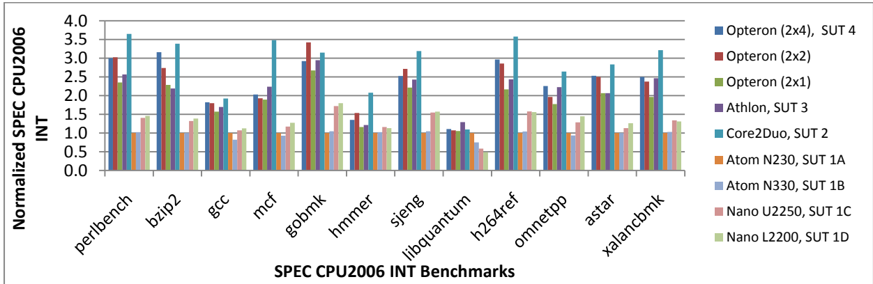
Figure 1. Per-core SPEC CPU2006 integer performance normalized to the Atom N230 for the systems (embedded, mobile, desktop, and server processors) from Table 1 plus two legacy Opteron servers.
